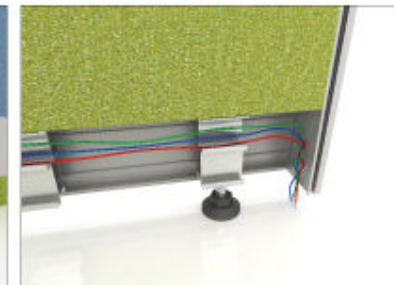
Wire Trunking
